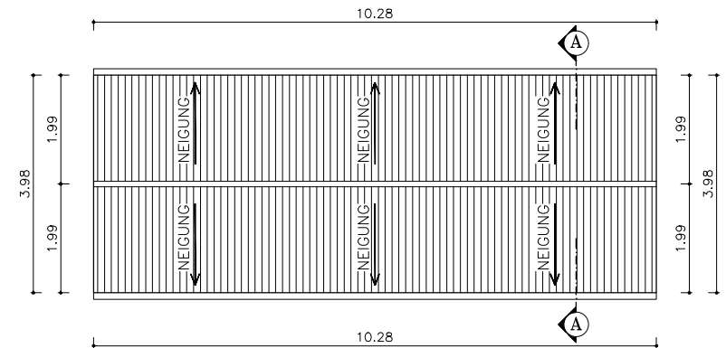
● Dachplan
