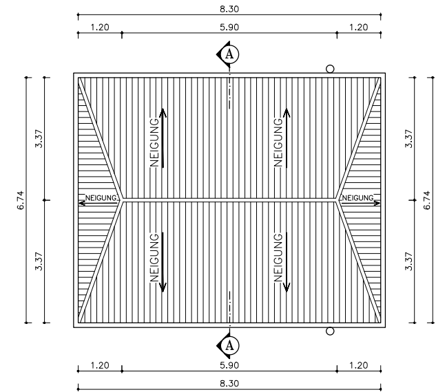
● Dachplan
