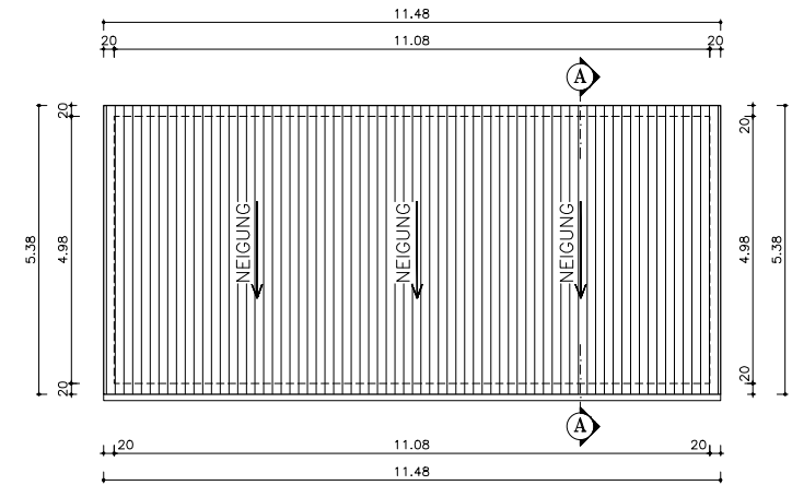
● Dachplan
