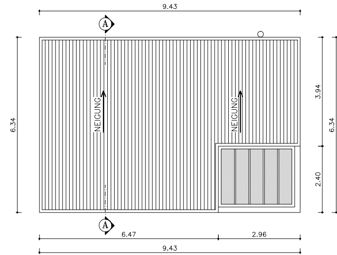
● Dachplan
