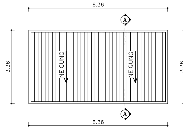
● Dachplan
