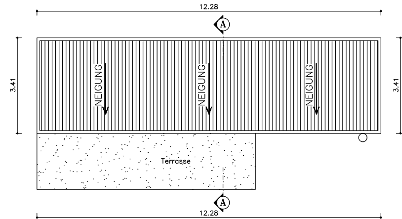
● Dachplan
