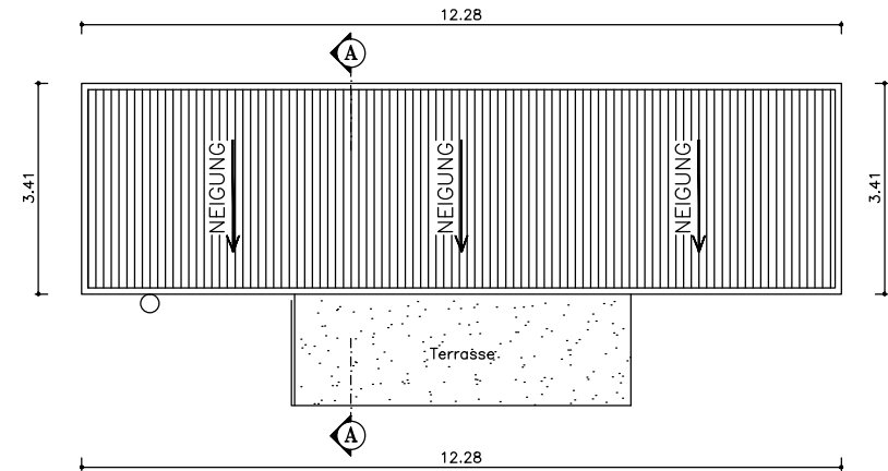
● Dachplan
